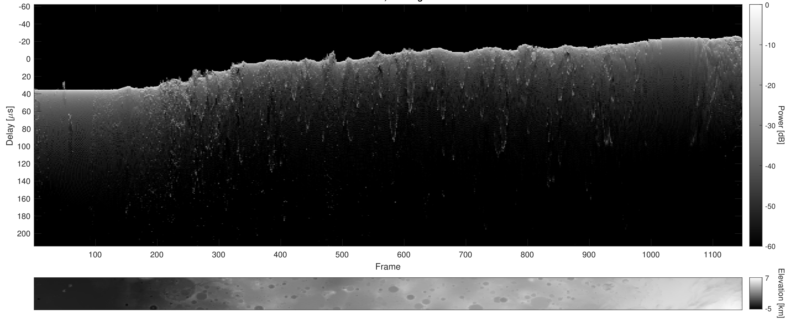
Orbit 11109, Cluttergram
