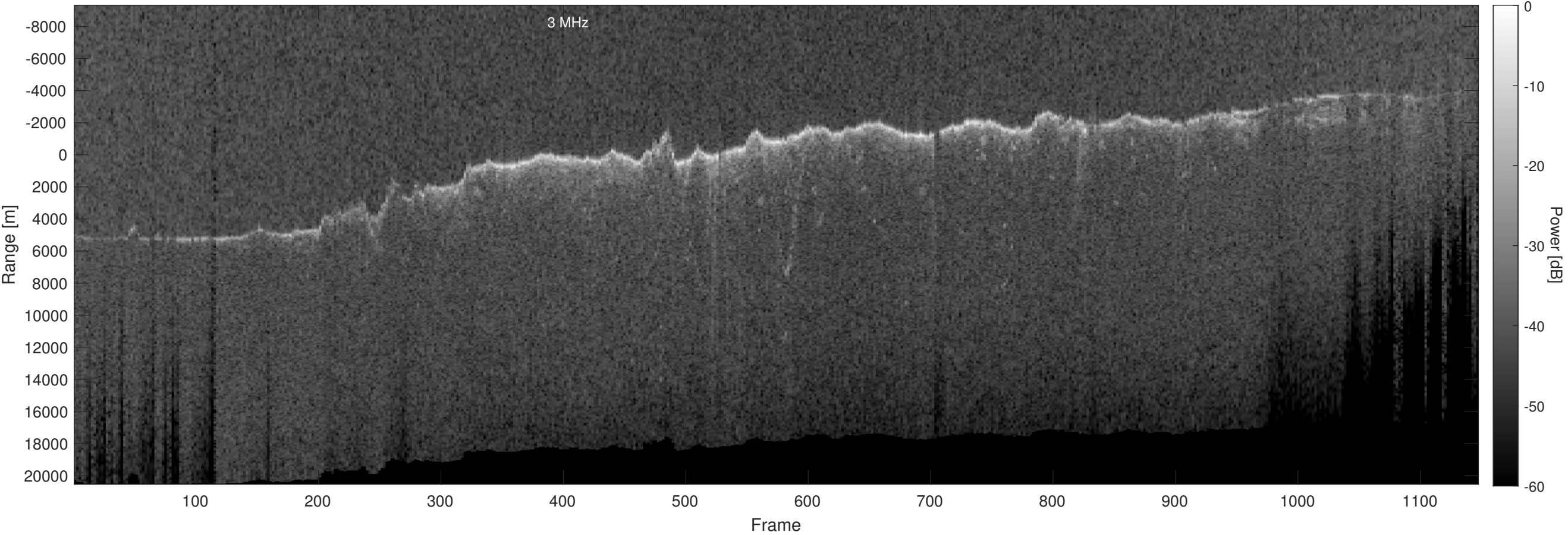
Orbit 11109, Optimized, Window, Depth-Corrected, Channel 2
