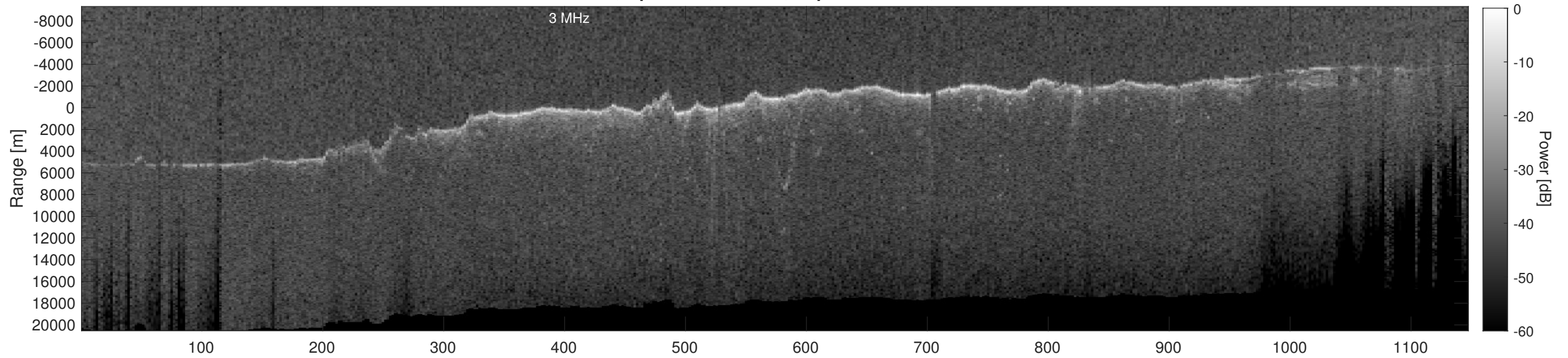
Orbit 11109, Depth-Corrected Cluttergram
