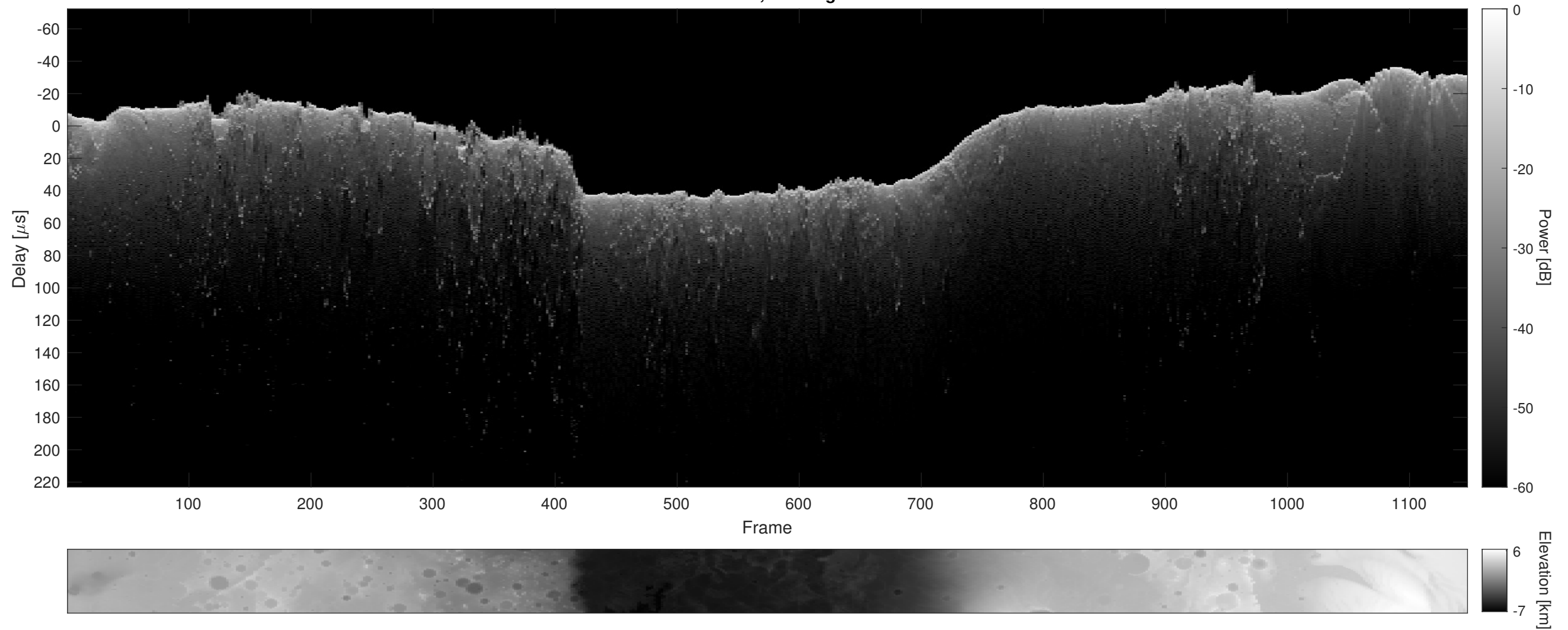
Orbit 11110, Cluttergram
