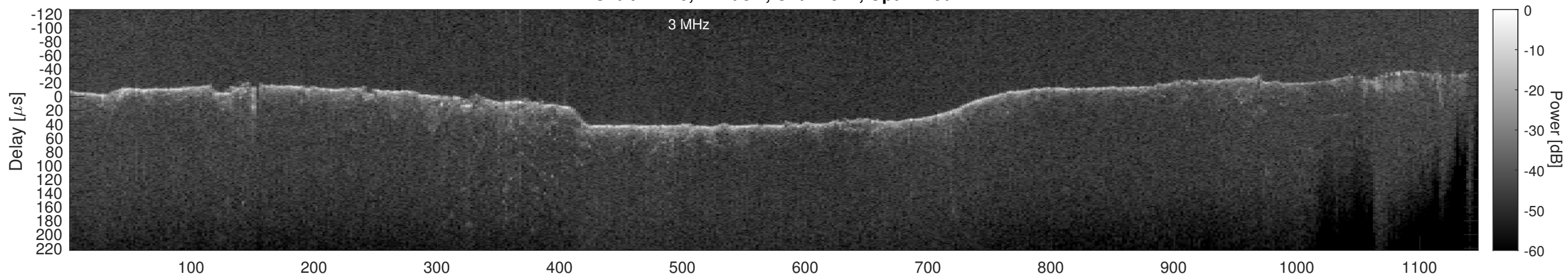
Orbit 11110, Cluttergram
