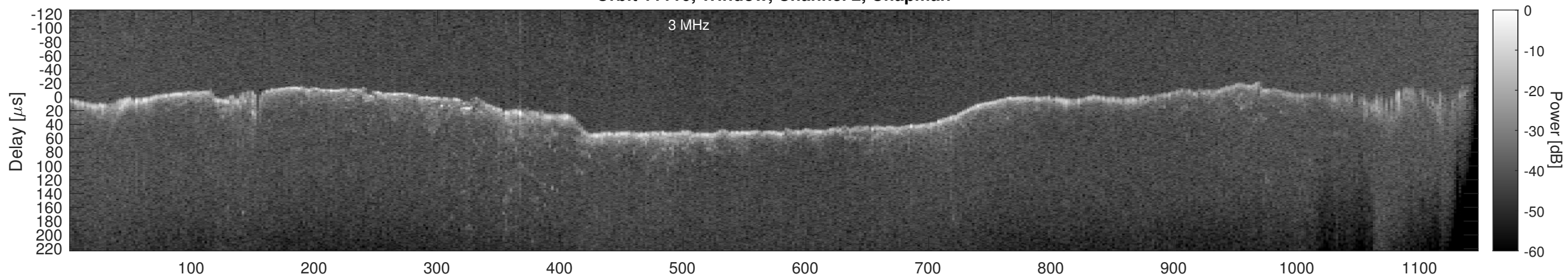
Orbit 11110, Window, Channel 2, Optimized
