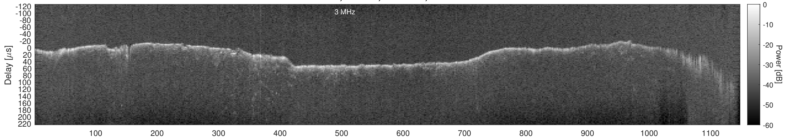
Orbit 11110, Window, Channel 2, Chapman
