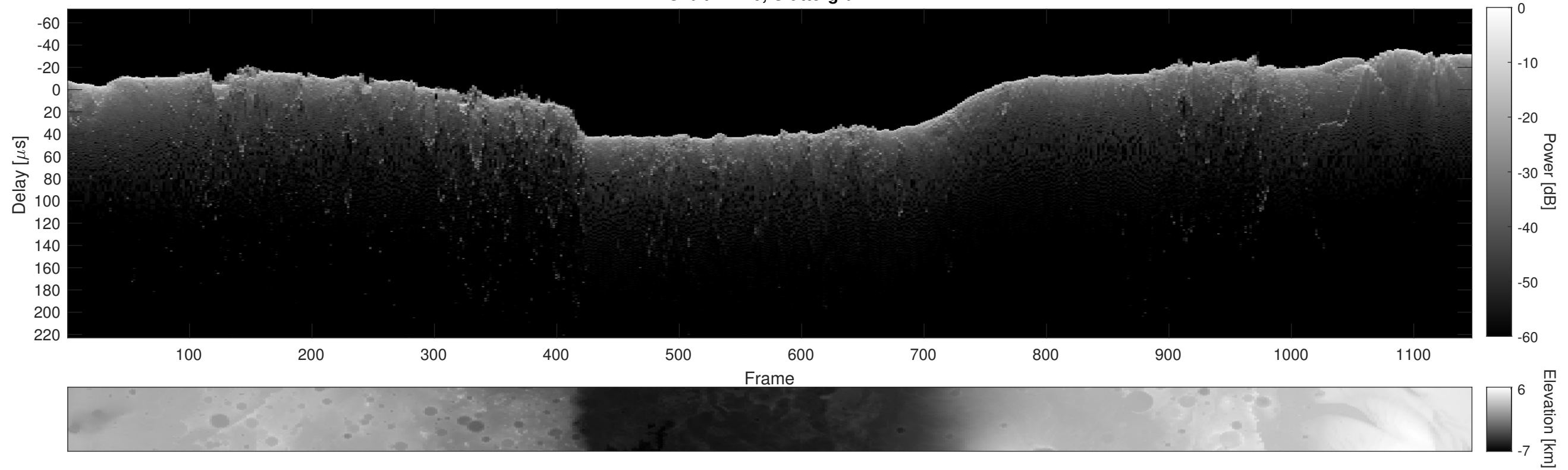
Orbit 11110, Cluttergram
