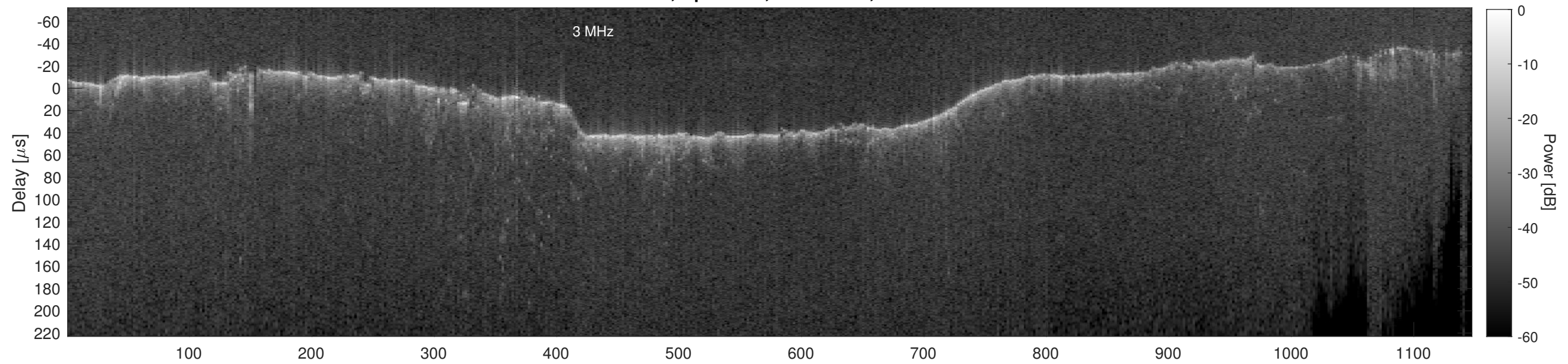
Orbit 11110, Cluttergram
