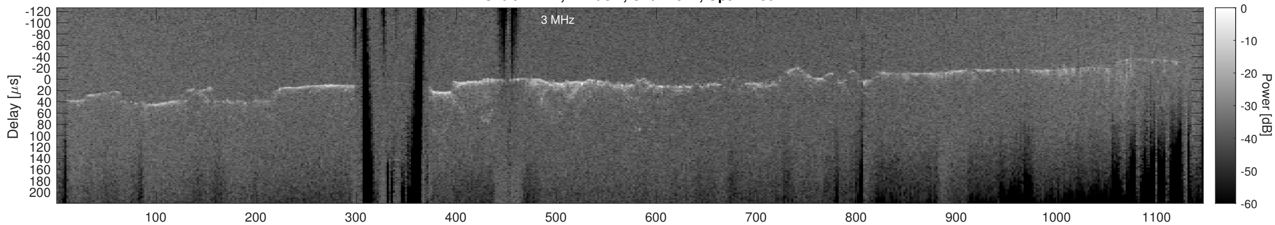
Orbit 11111, Cluttergram
