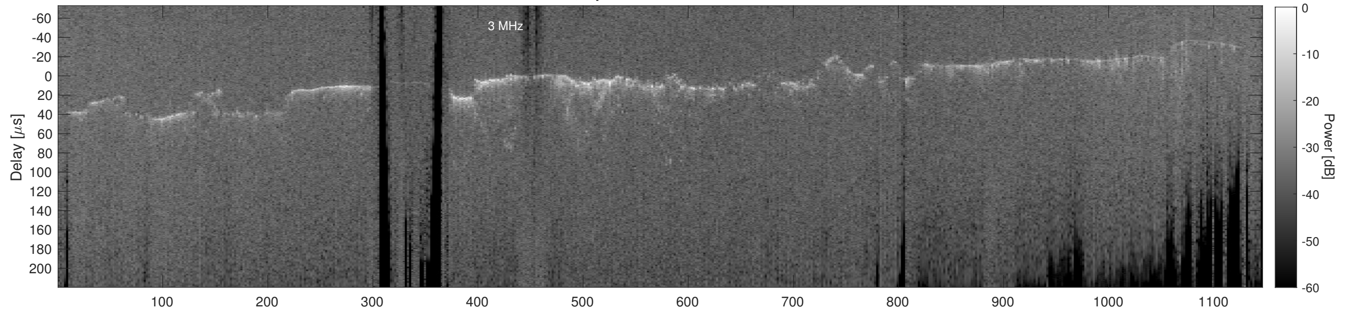
Orbit 11111, Cluttergram
