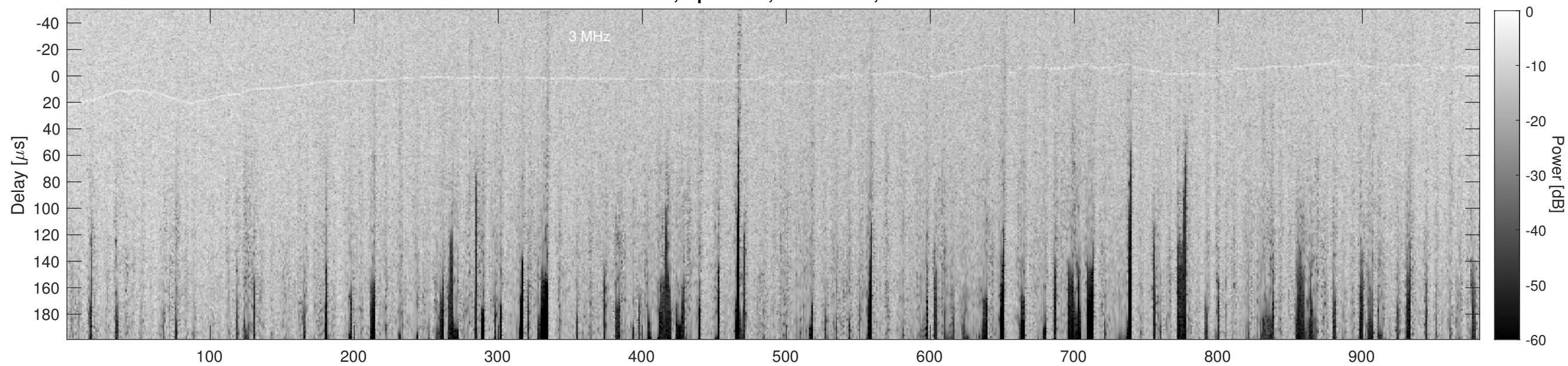
Orbit 11112, Cluttergram
