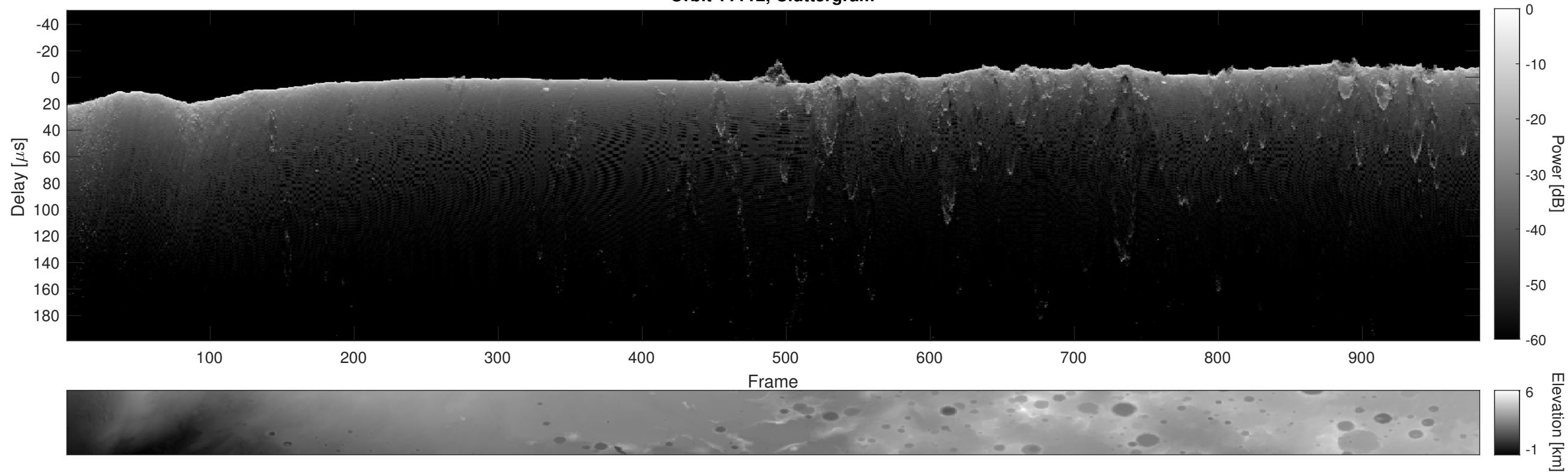
Orbit 11112, Cluttergram
