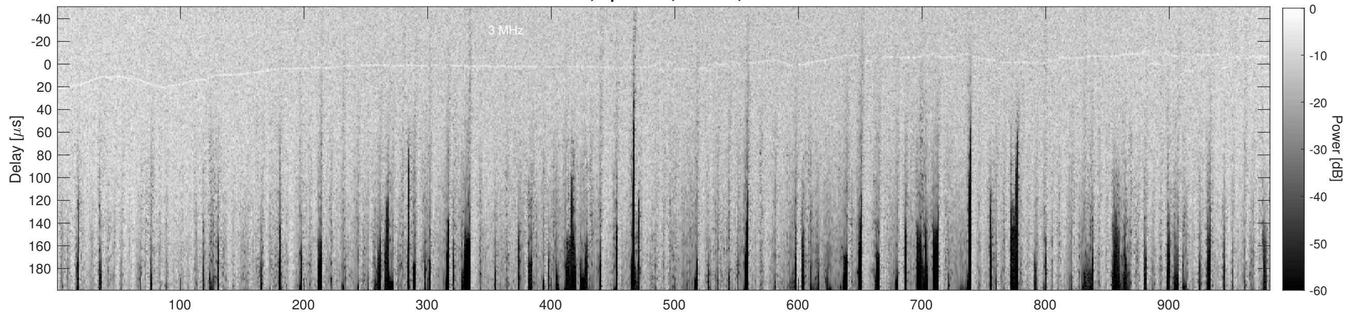
Orbit 11112, Cluttergram
