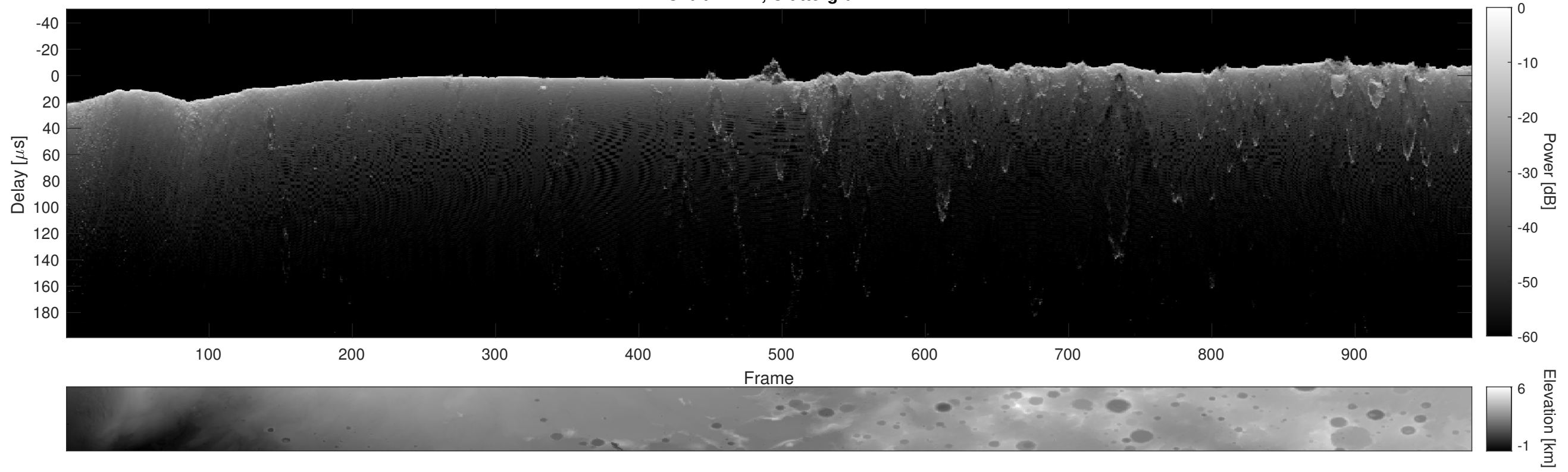
Orbit 11112, Cluttergram
