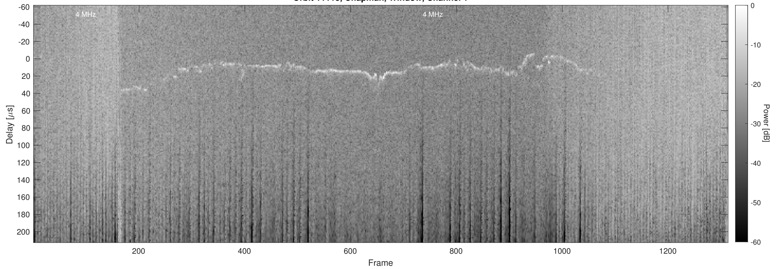
Orbit 11113, Chapman, Window, Channel 2
