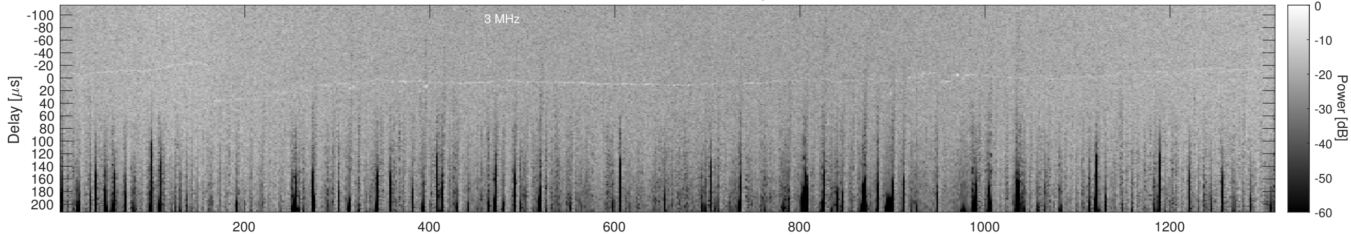
Orbit 11113, Cluttergram
