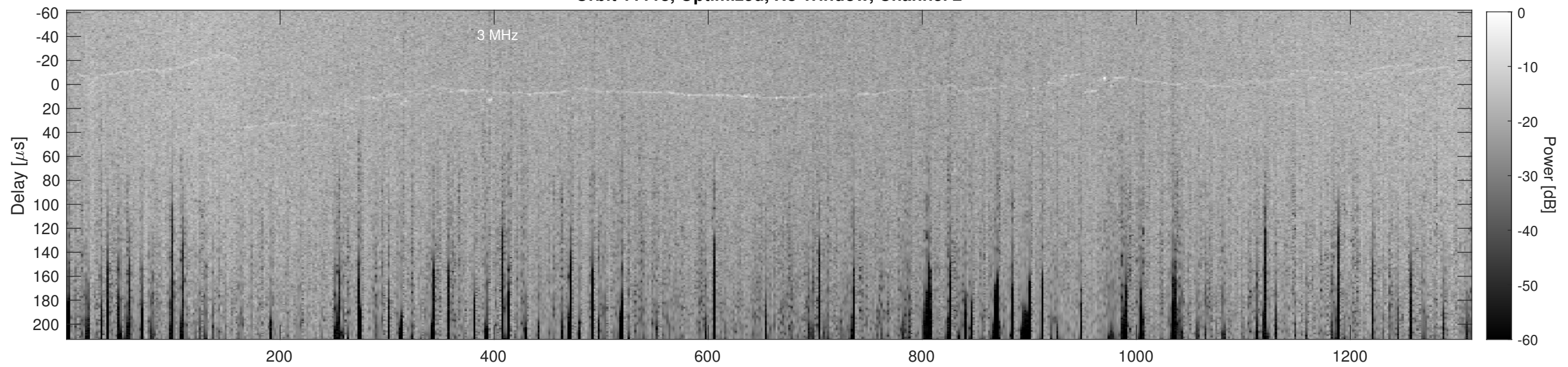
Orbit 11113, Cluttergram
