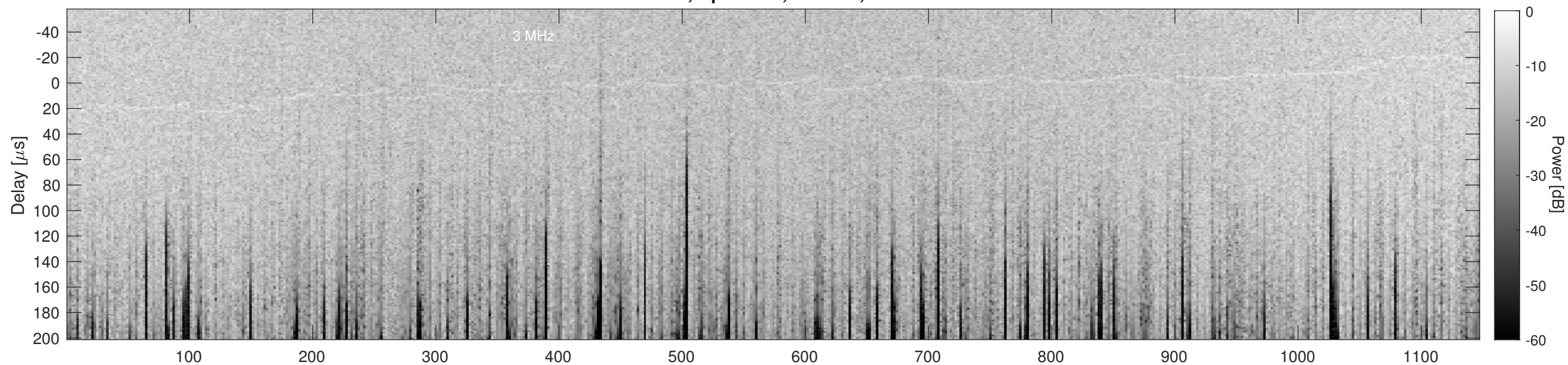
Orbit 11114, Cluttergram
