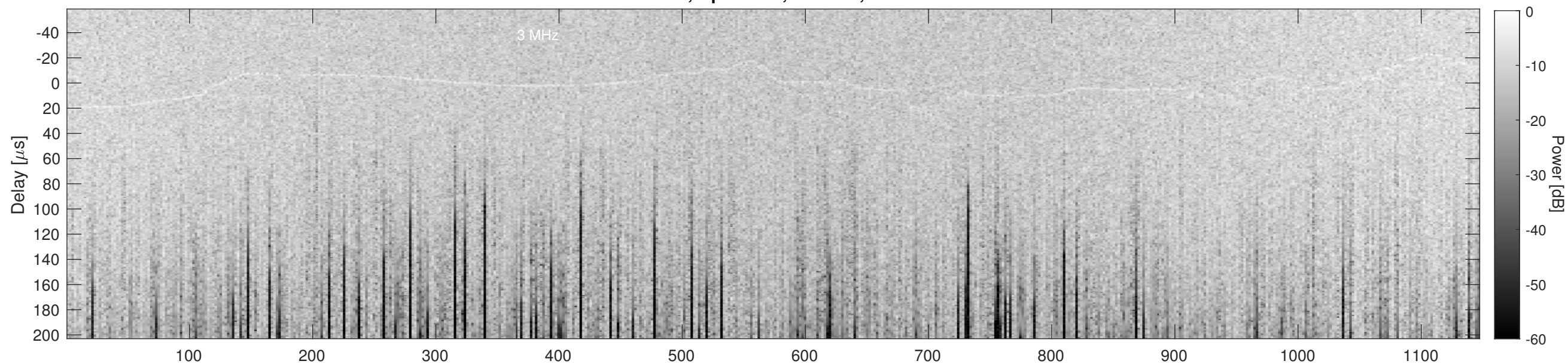
Orbit 11115, Cluttergram
