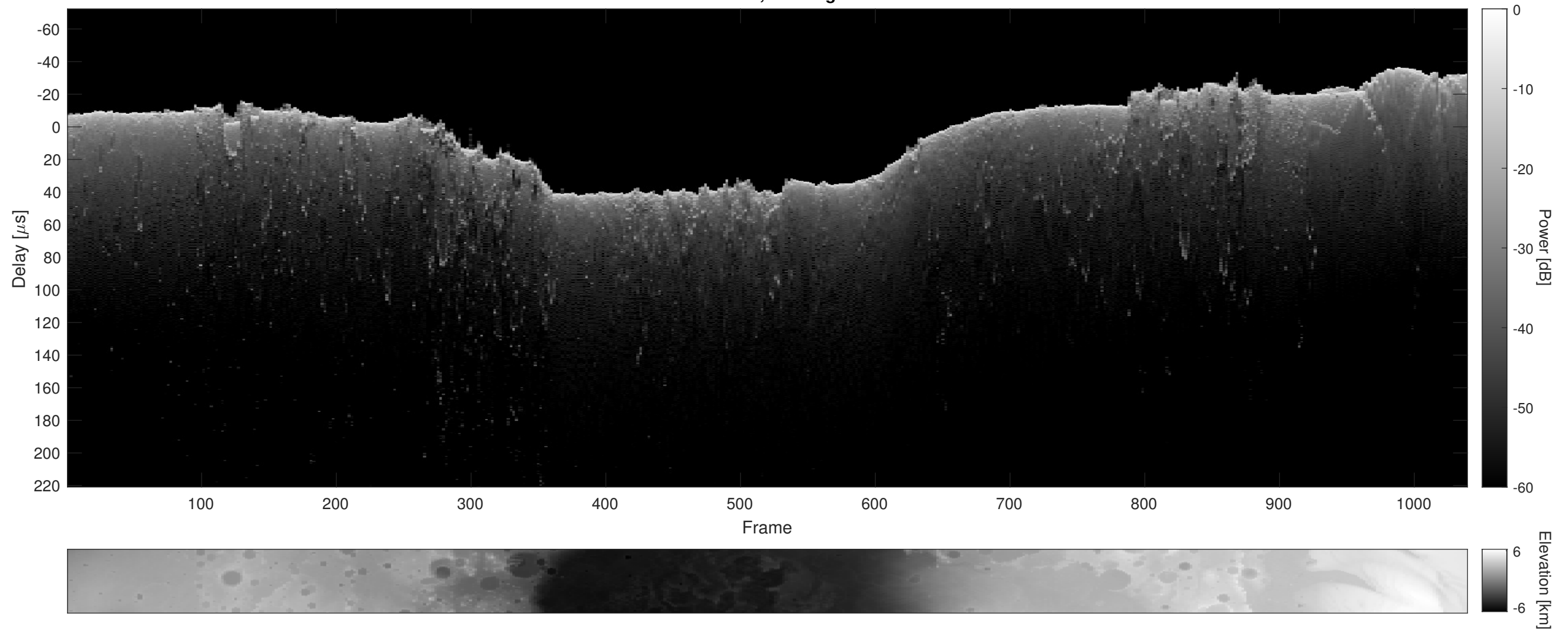
Orbit 11117, Cluttergram
