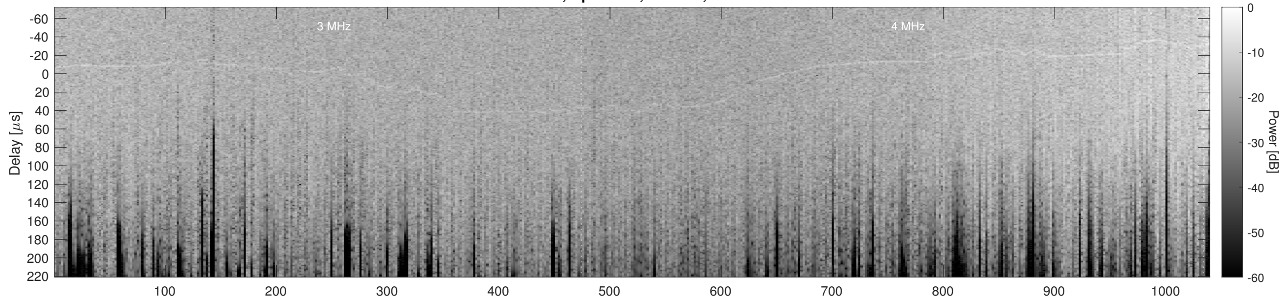
Orbit 11117, Optimized, Window, Channel 2
