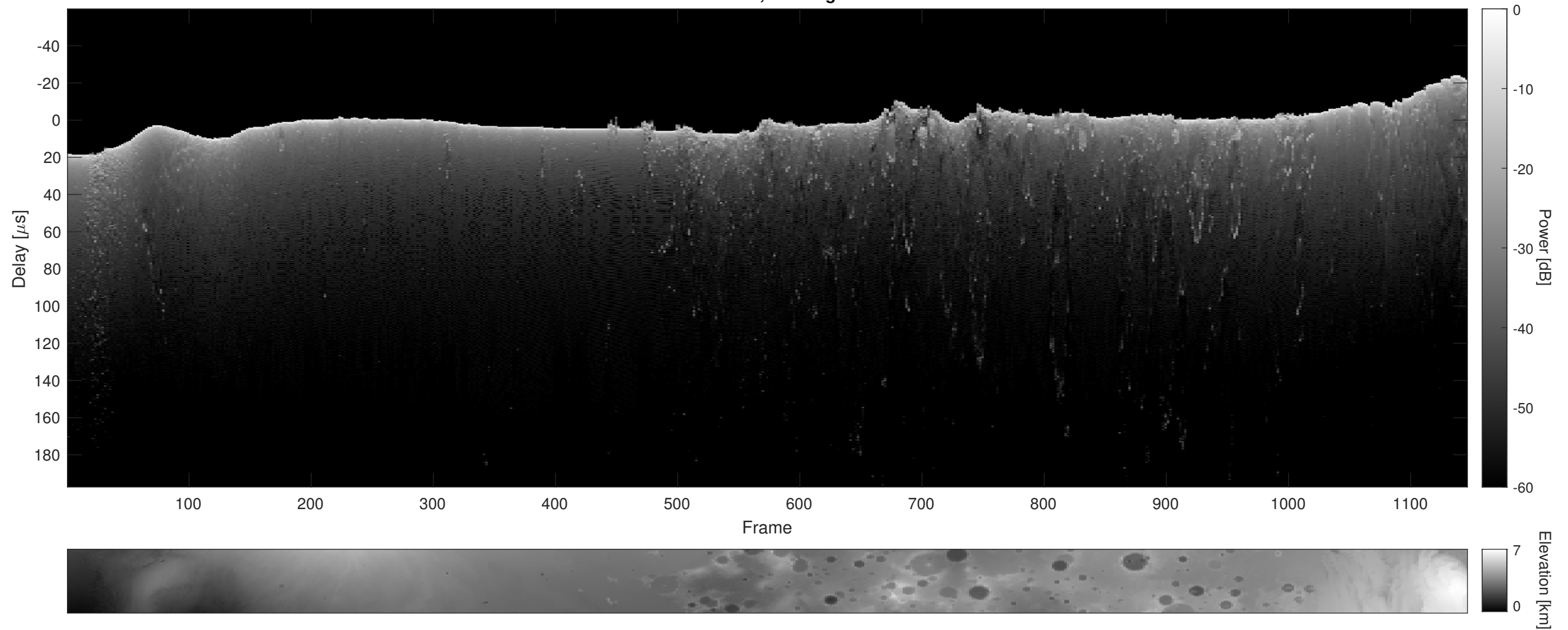
Orbit 11119, Cluttergram
