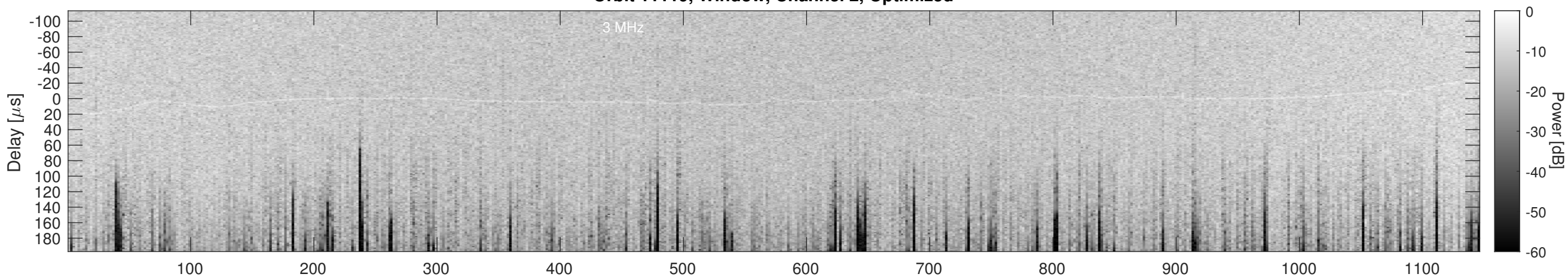
Orbit 11119, Cluttergram
