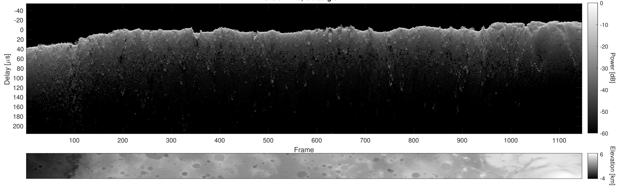
Orbit 11120, Cluttergram
