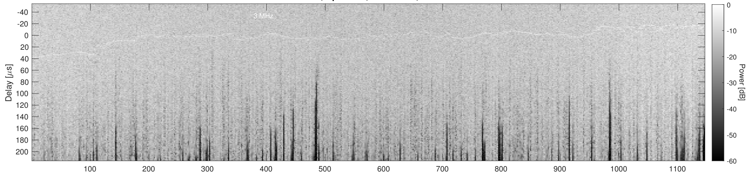
Orbit 11120, Cluttergram
