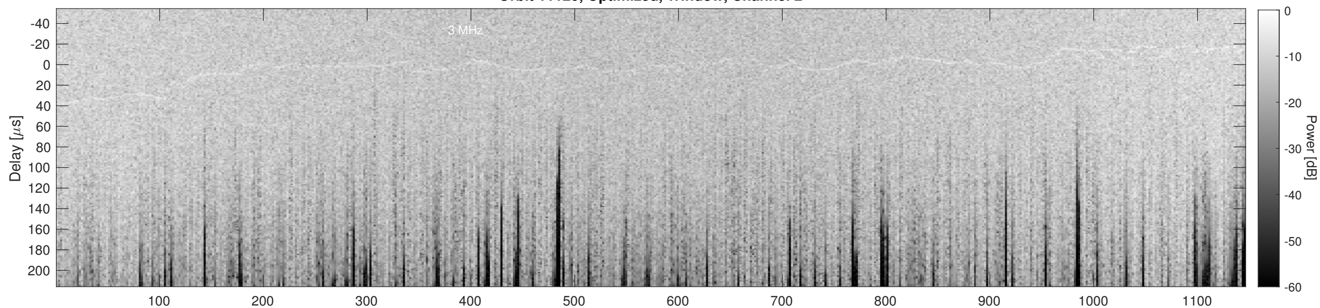
Orbit 11120, Cluttergram
