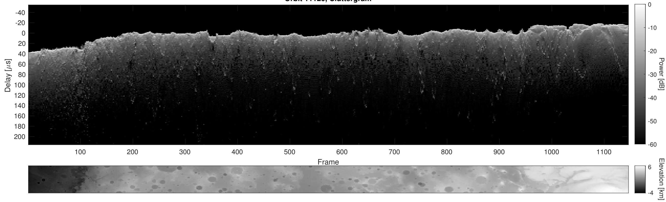
Orbit 11120, Cluttergram
