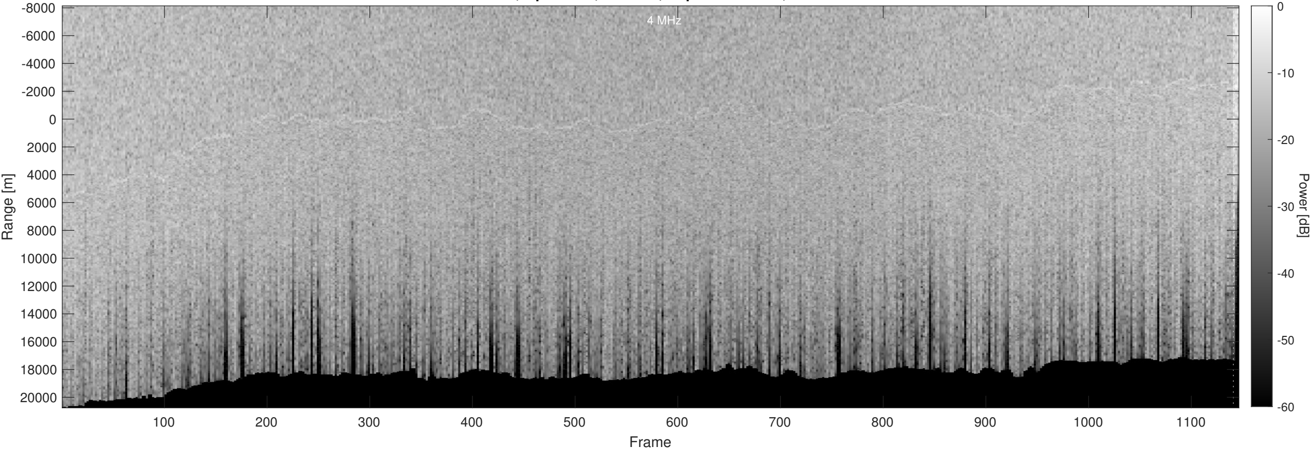
Orbit 11120, Optimized, Window, Depth-Corrected, Channel 2
