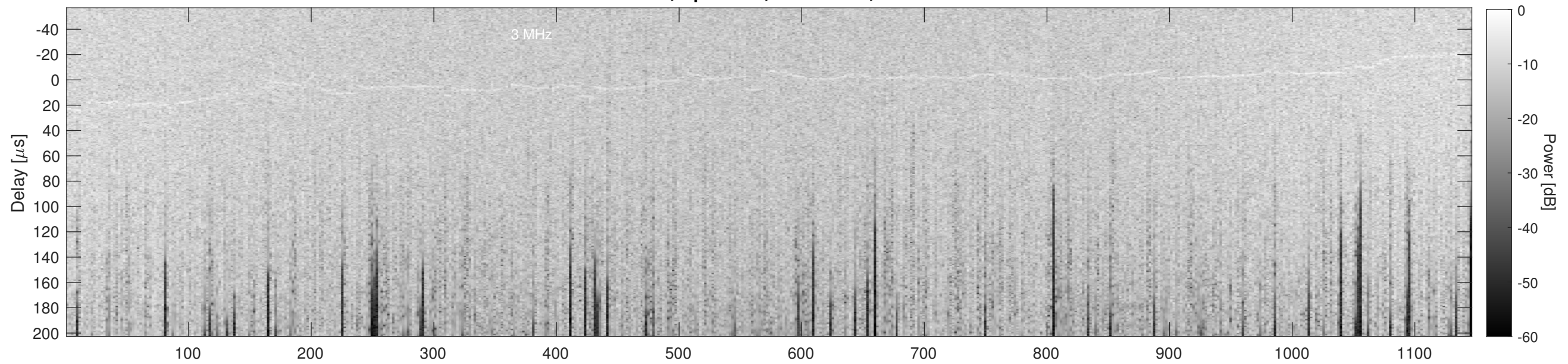
Orbit 11121, Cluttergram
