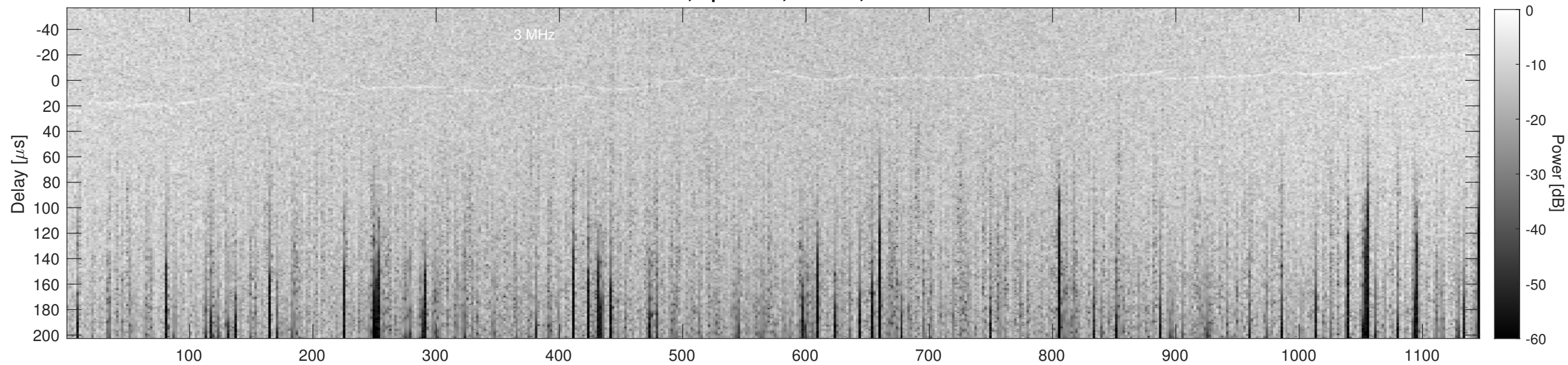
Orbit 11121, Cluttergram
