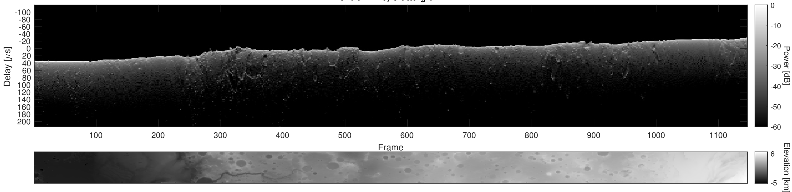
Orbit 11123, Cluttergram
