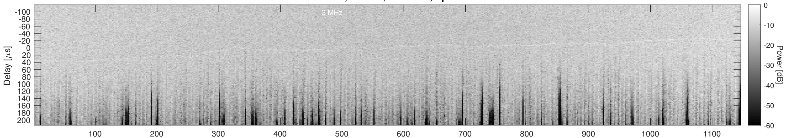
Orbit 11123, Cluttergram
