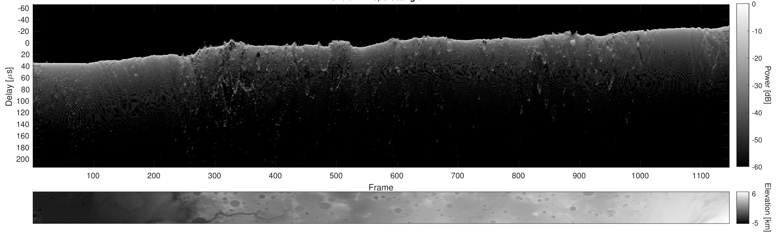
Orbit 11123, Cluttergram
