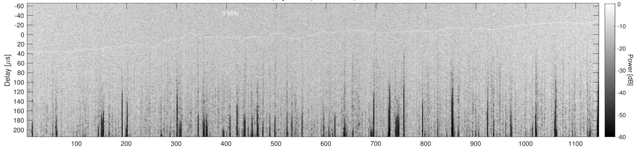
Orbit 11123, Cluttergram
