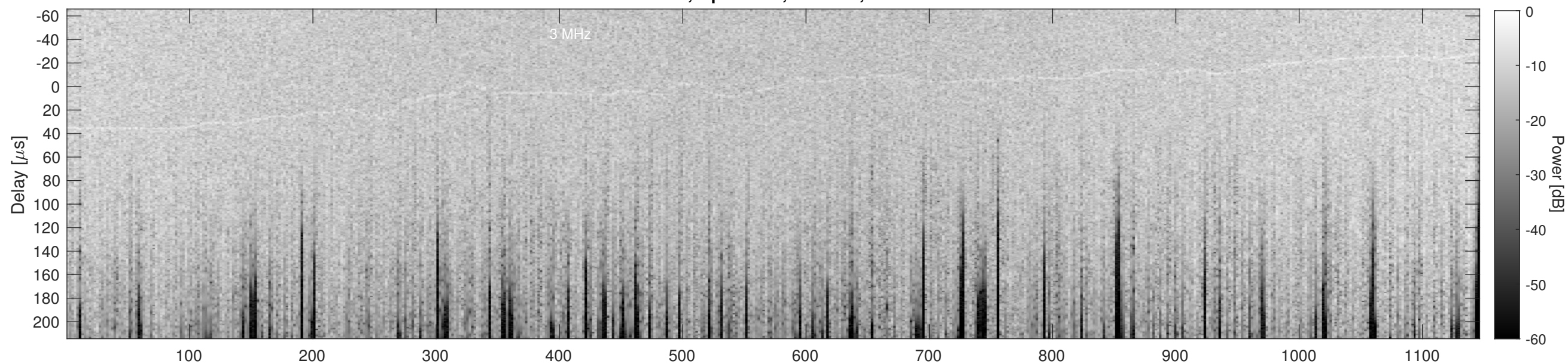
Orbit 11123, Cluttergram
