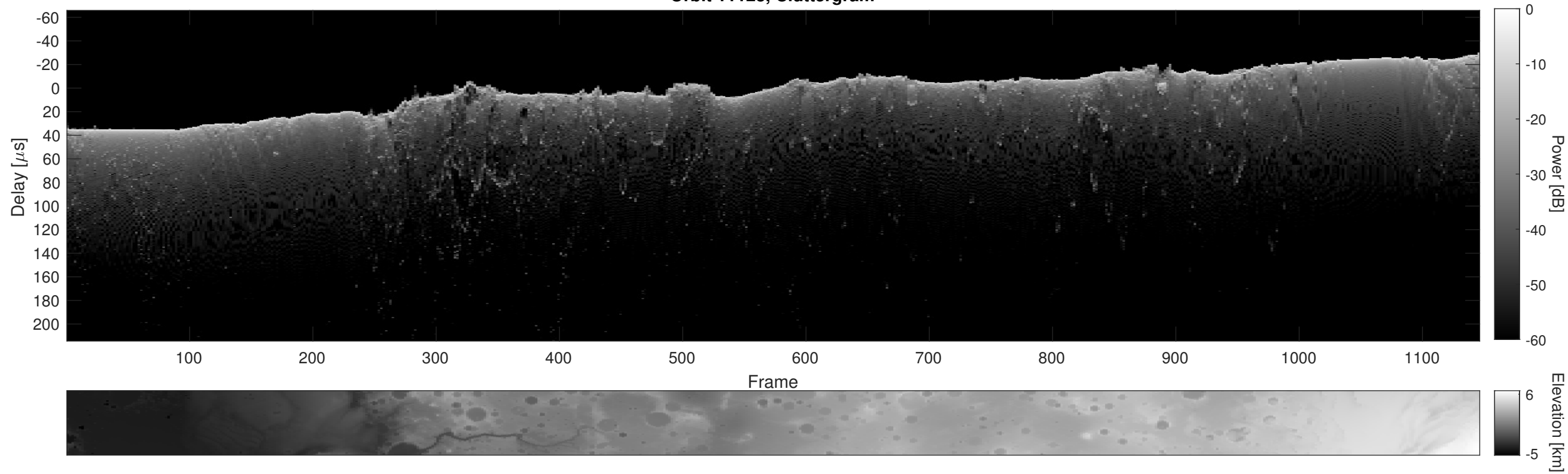
Orbit 11123, Cluttergram
