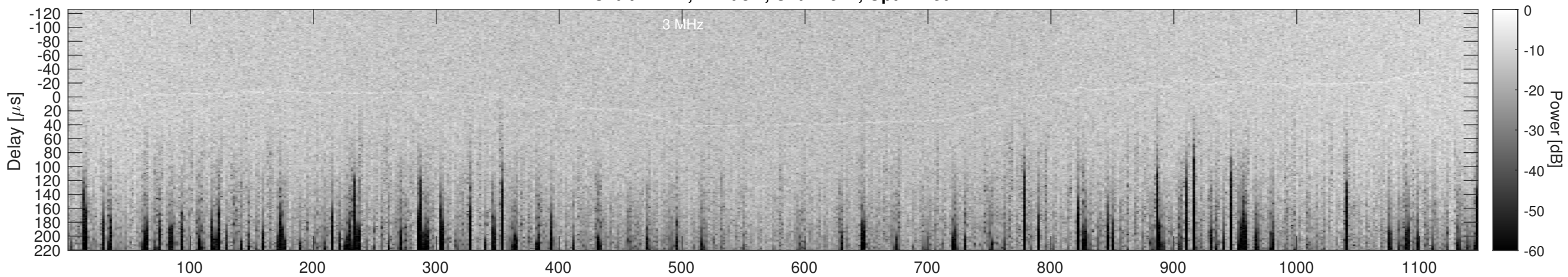
Orbit 11124, Cluttergram
