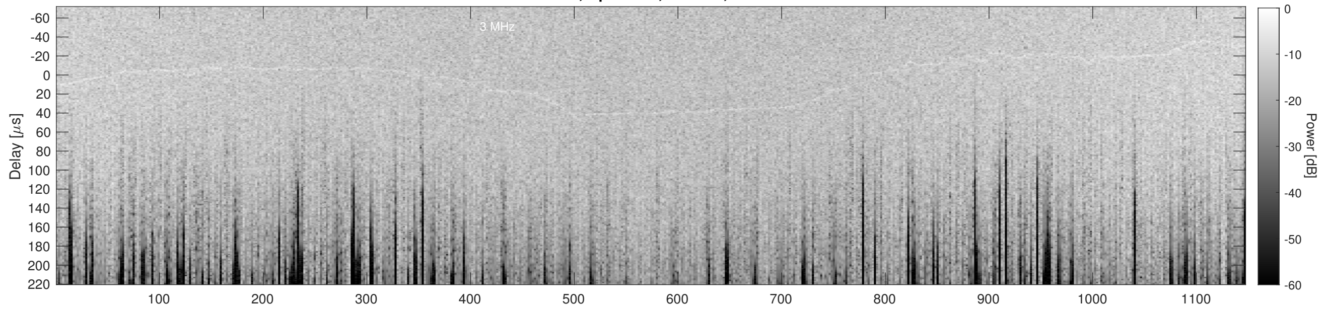
Orbit 11124, Cluttergram
