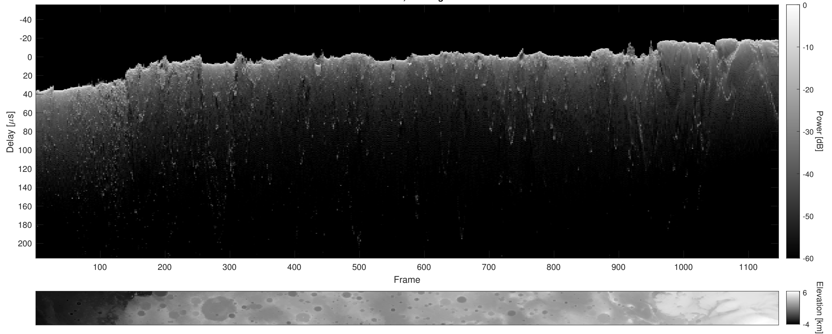
Orbit 11127, Cluttergram
