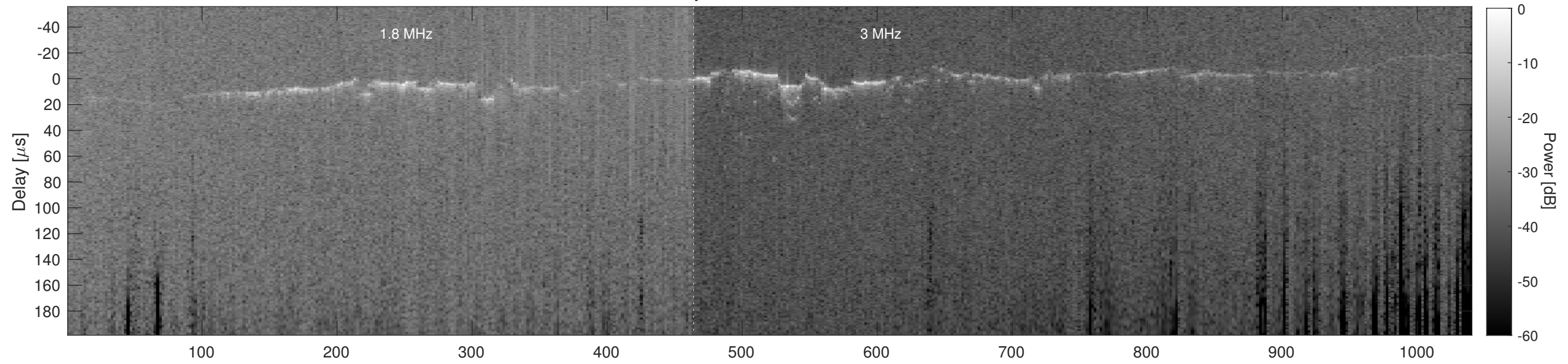
Orbit 11128, Cluttergram
