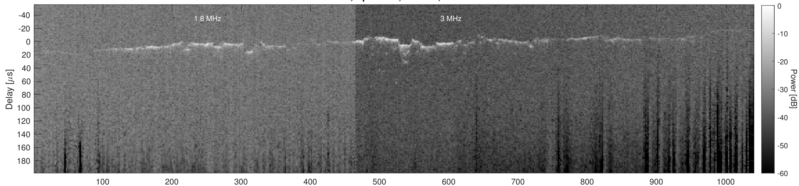
Orbit 11128, Cluttergram
