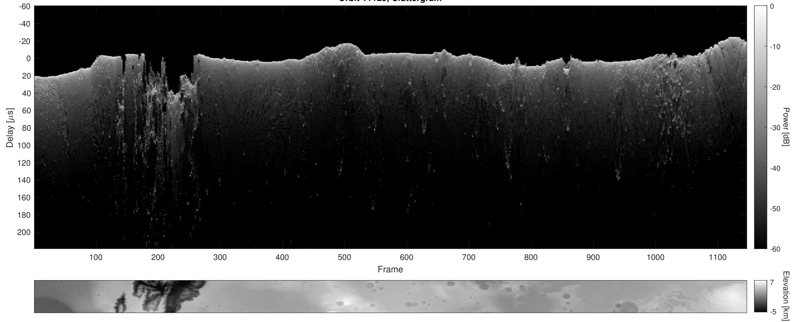
Orbit 11129, Cluttergram
