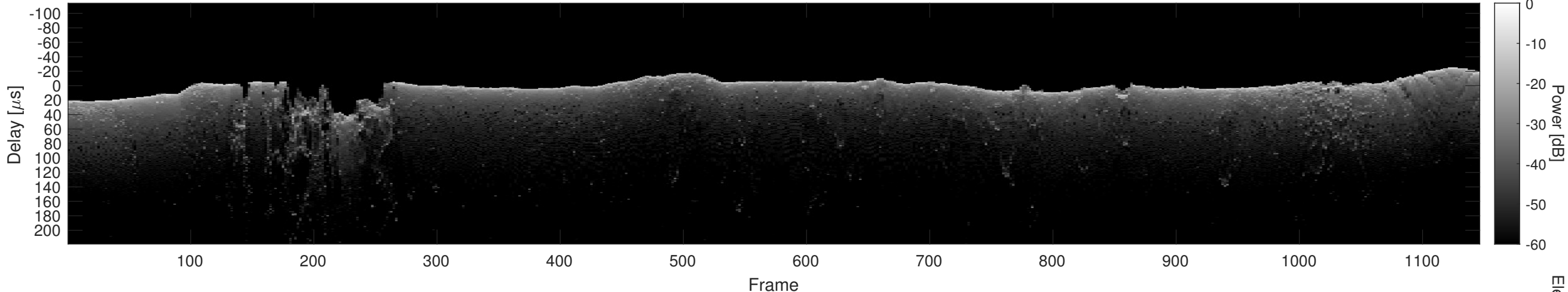
Orbit 11129, Cluttergram
