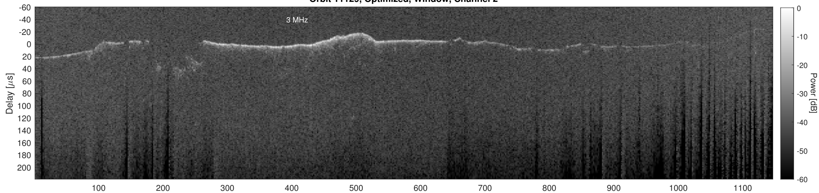
Orbit 11129, Cluttergram
