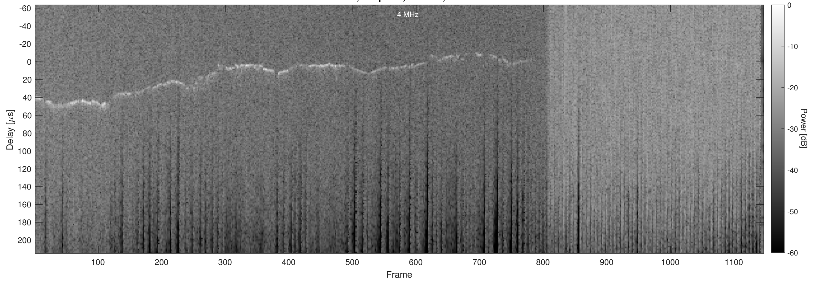
Orbit 11130, Chapman, Window, Channel 2
