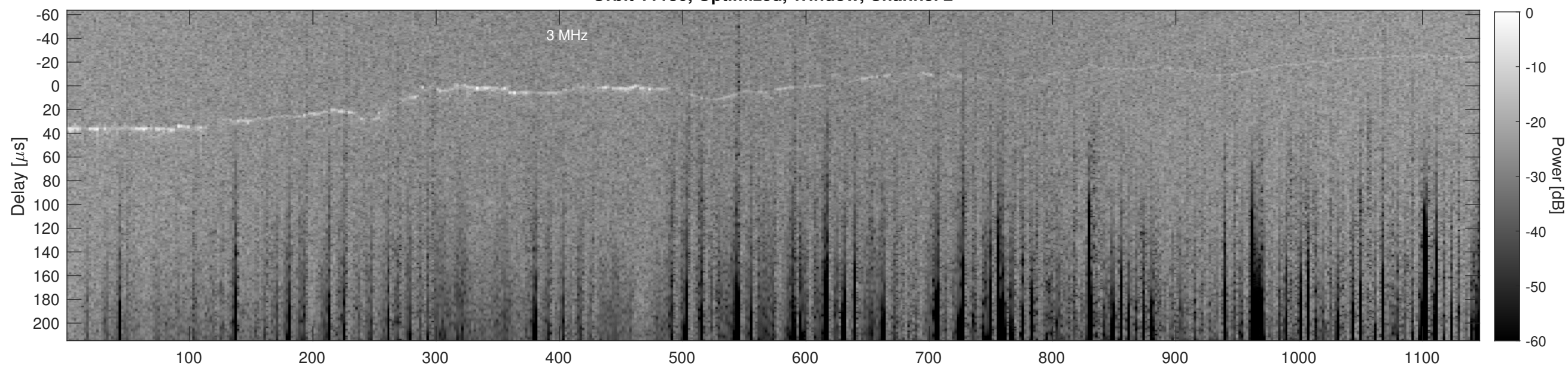
Orbit 11130, Cluttergram
