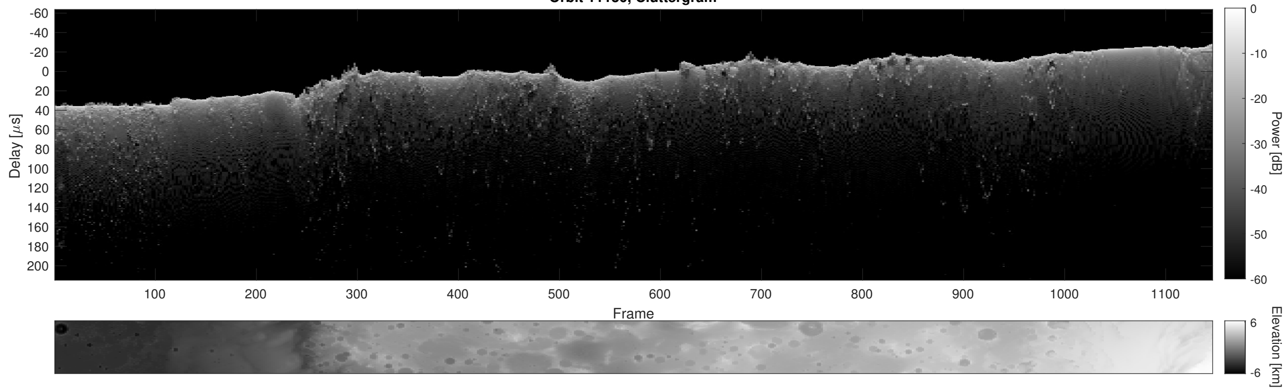
Orbit 11130, Cluttergram
