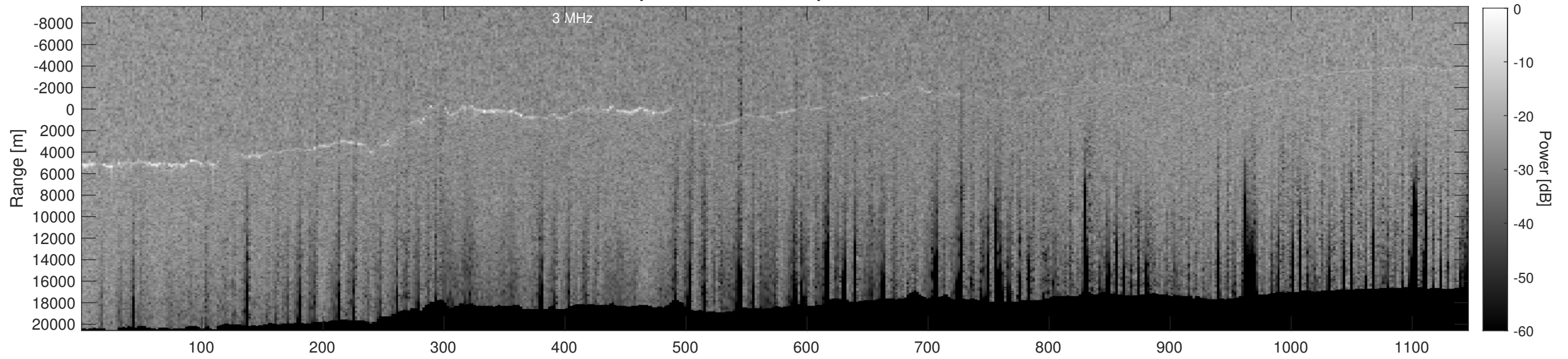
Orbit 11130, Depth-Corrected Cluttergram
