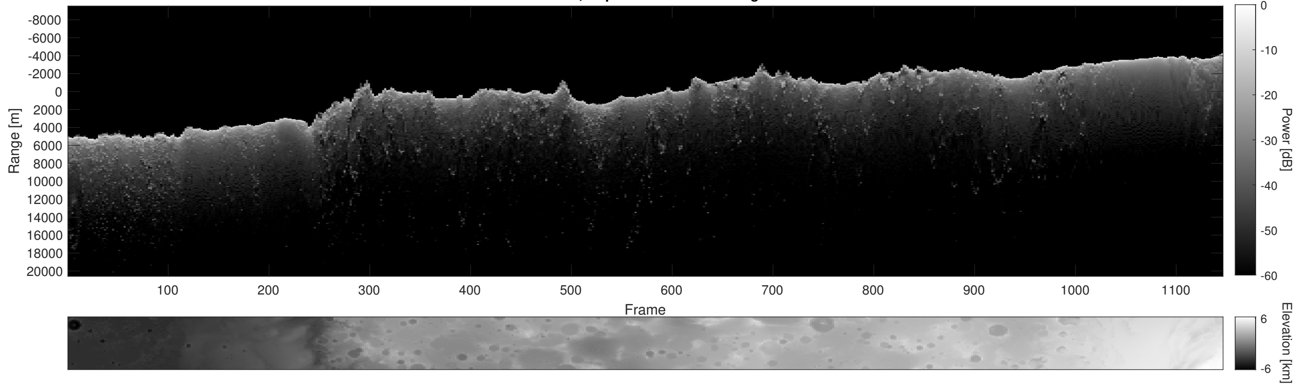
Orbit 11130, Depth-Corrected Cluttergram
