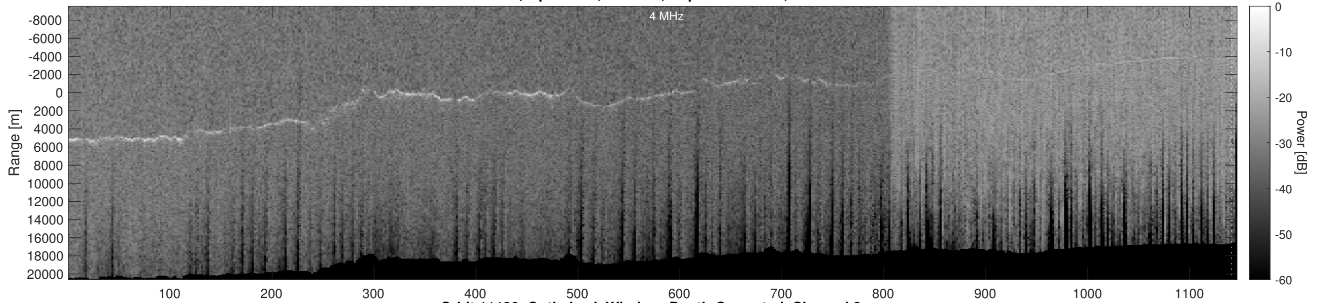
Orbit 11130, Optimized, Window, Depth-Corrected, Channel 2
