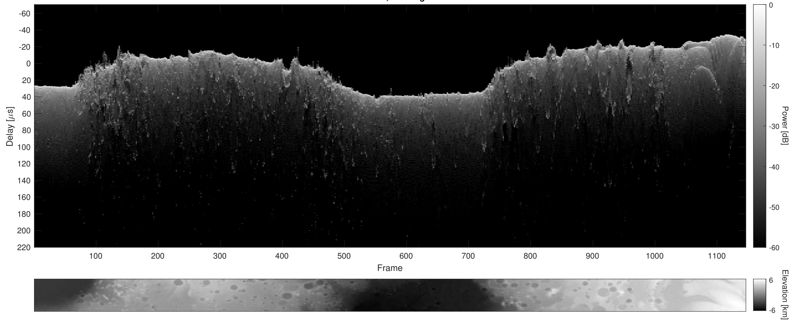
Orbit 11131, Cluttergram
