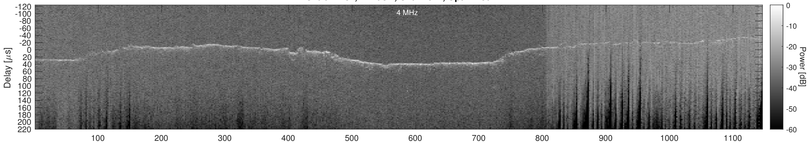
Orbit 11131, Cluttergram
