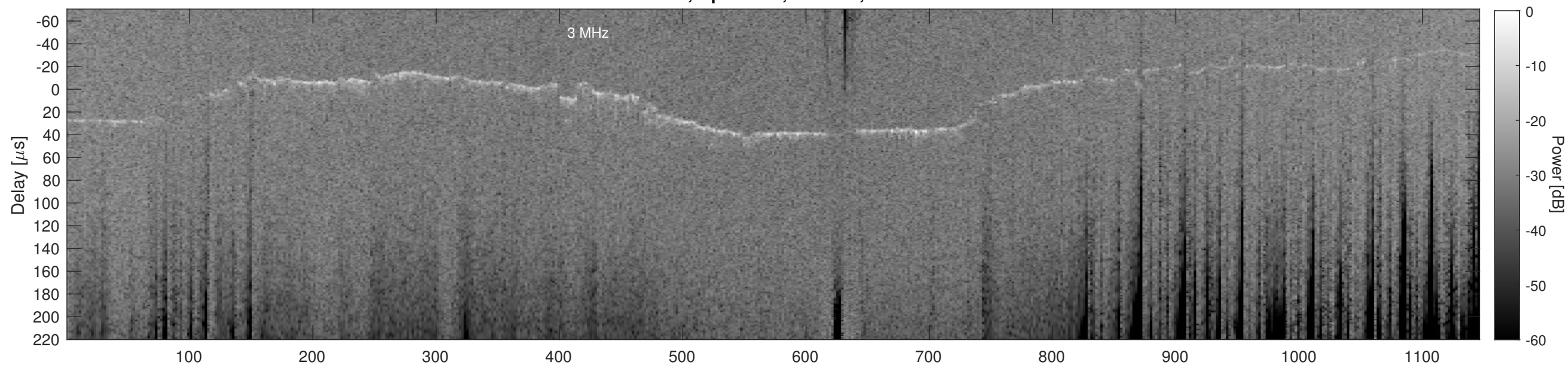
Orbit 11131, Cluttergram
