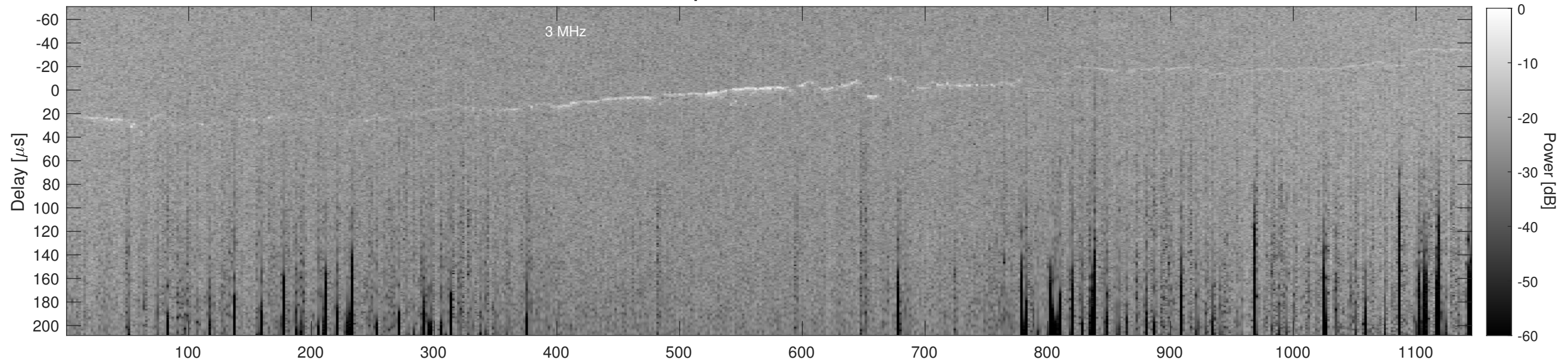
Orbit 11132, Cluttergram
