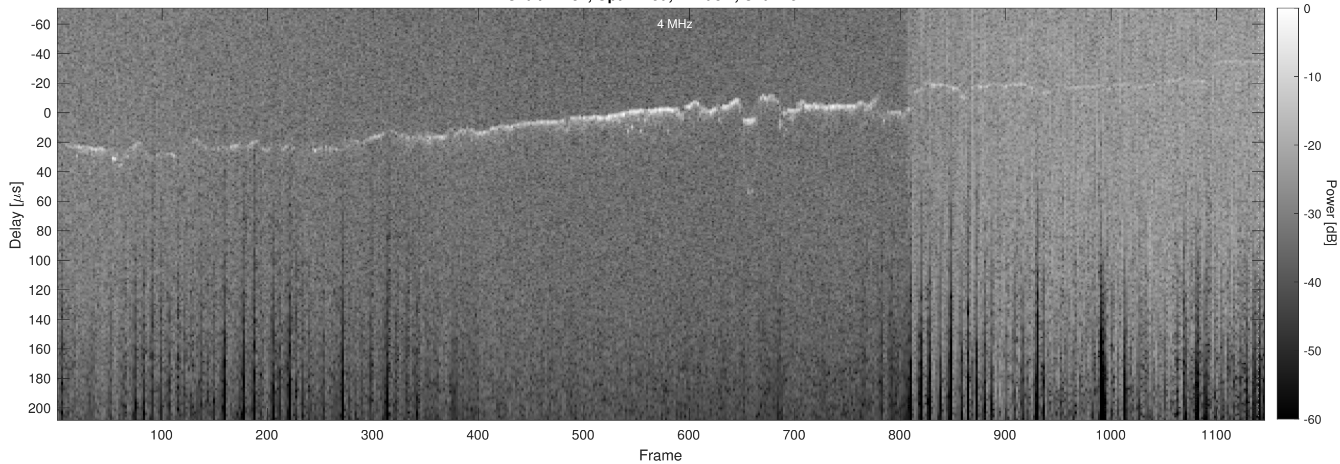
Orbit 11132, Optimized, Window, Channel 2
