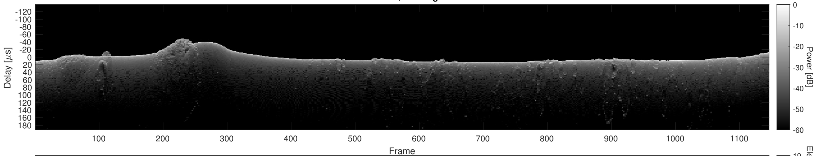
Orbit 11133, Cluttergram
