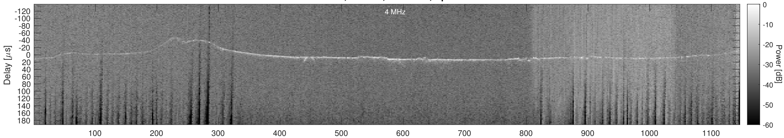
Orbit 11133, Cluttergram
