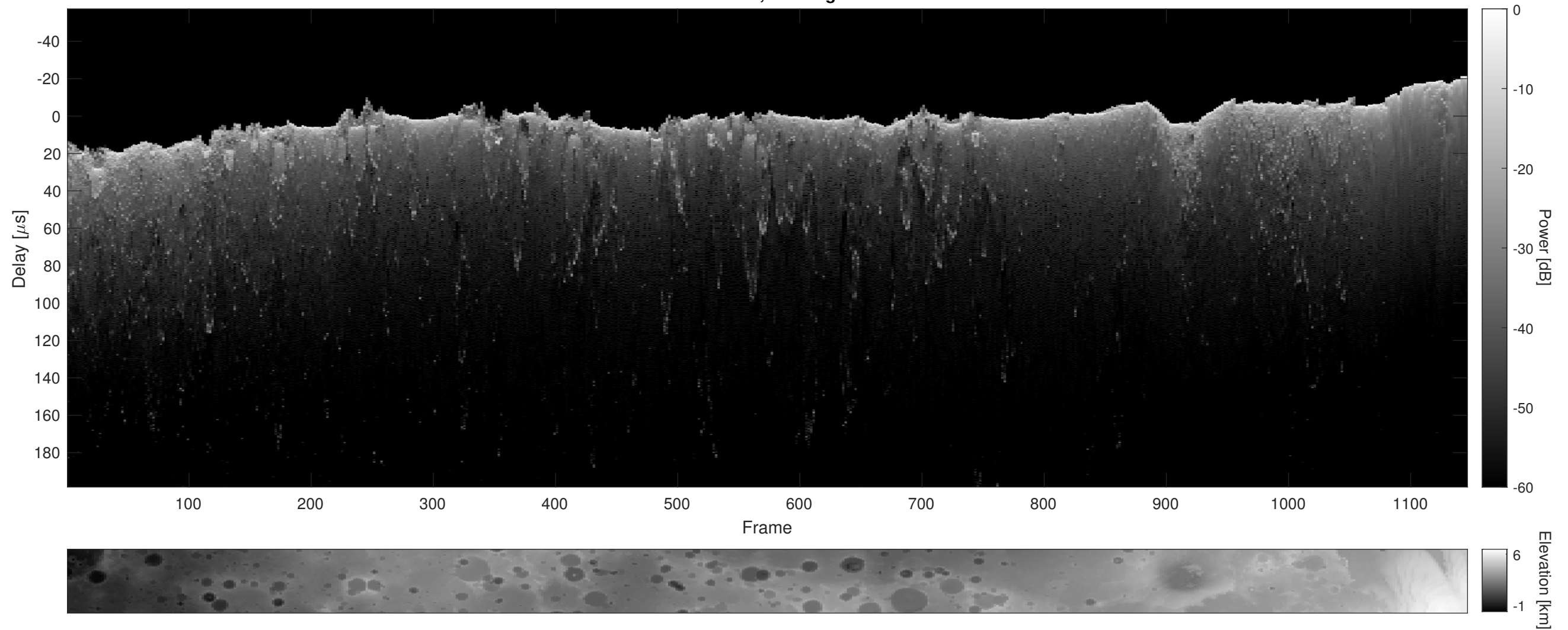
Orbit 11135, Cluttergram
