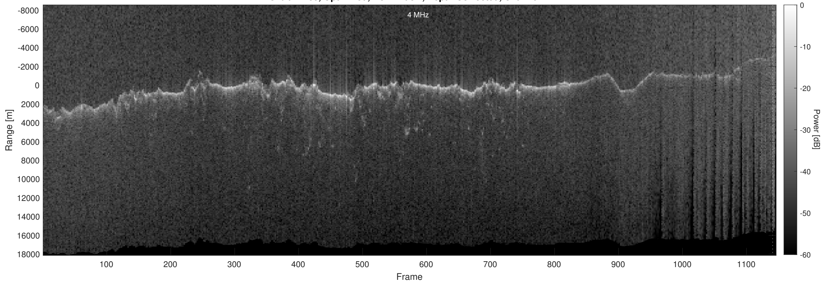
Orbit 11135, Optimized, No Window, Depth-Corrected, Channel 2
