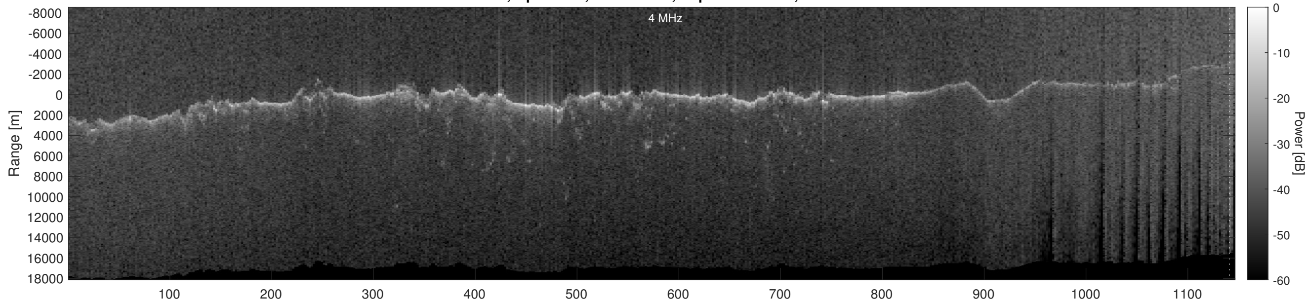
Orbit 11135, Optimized, No Window, Depth-Corrected, Channel 2
