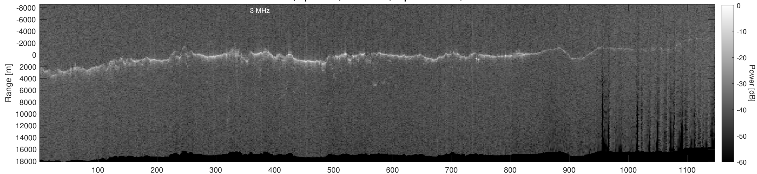
Orbit 11135, Depth-Corrected Cluttergram
