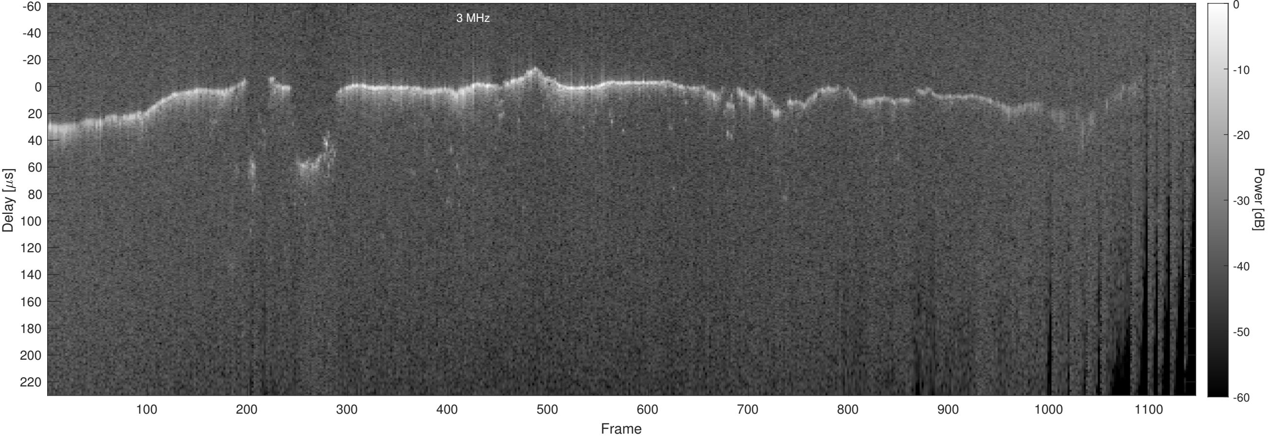
Orbit 11136, Chapman, No Window, Channel 2
