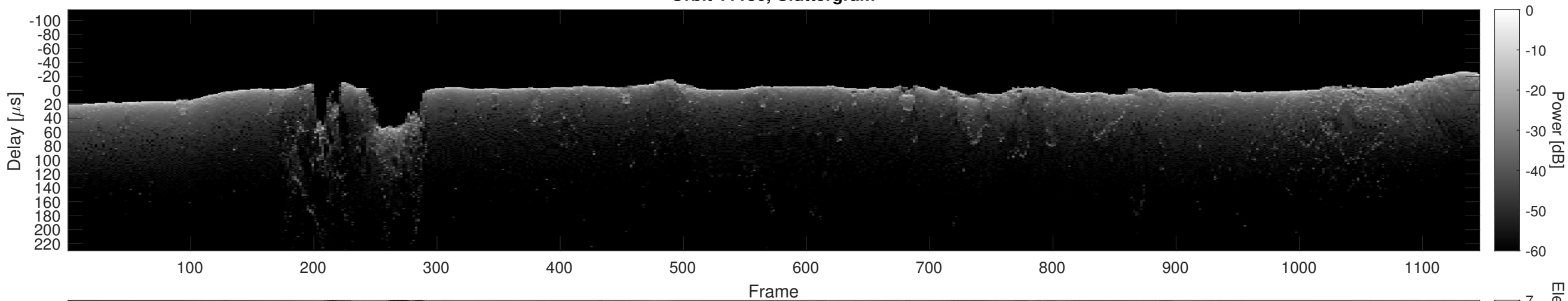
Orbit 11136, Cluttergram
