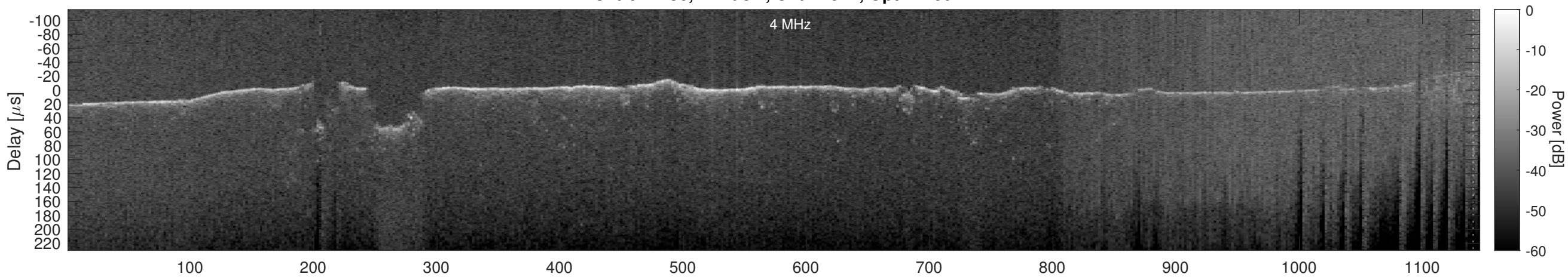
Orbit 11136, Cluttergram
