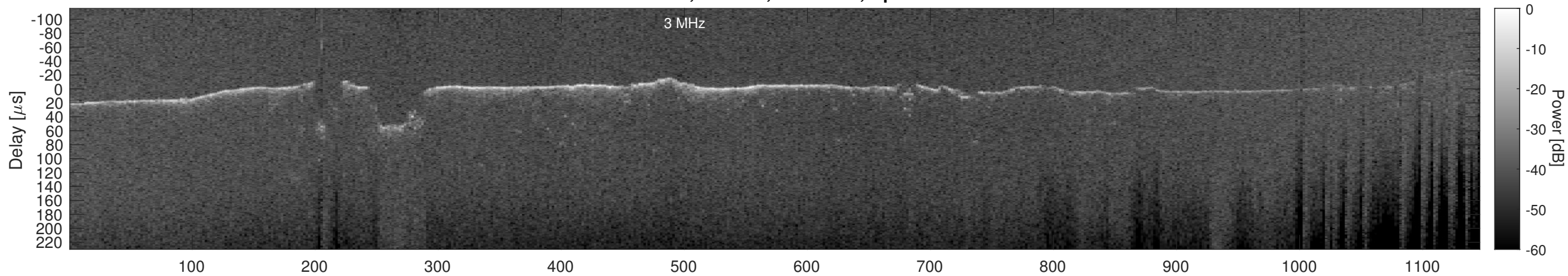
Orbit 11136, Cluttergram
